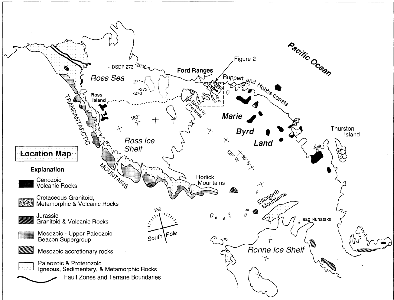
Figure 1. Geologic setting of Marie Byrd Land in West Antarctica showing the location of the Ford Ranges, the Ruppert and Hobbs Coasts, and Thurston Island. Drill sites of Deep Sea Drilling Project Leg 28 in the Ross Sea are shown. Geology is from Craddock et al. [1989].
